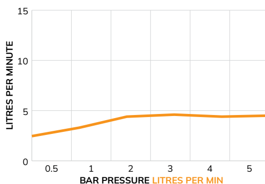
FLOW RATES
