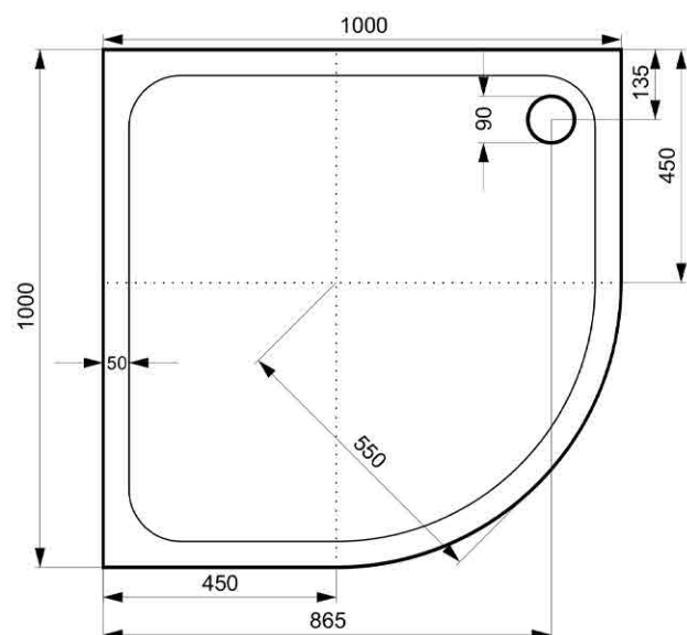
1000mm Quadrant
