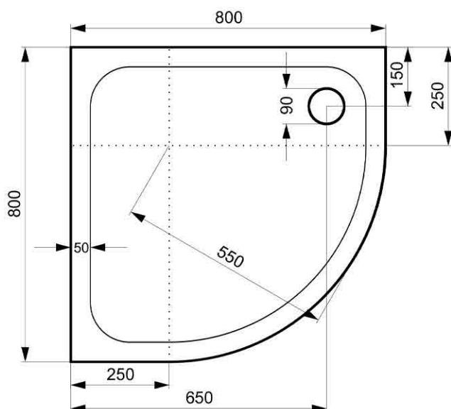
800mm Quadrant
